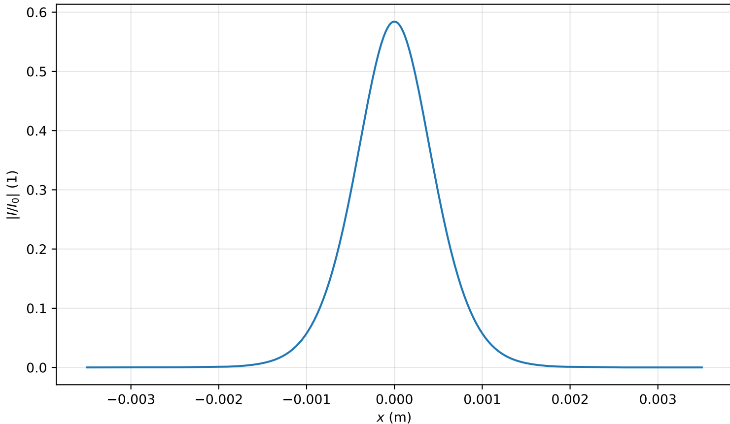
Intensity profile I(x, y = 0, z = 3.423m)/I_0 , P_{in}=0.6P_{cr} , artificial time
